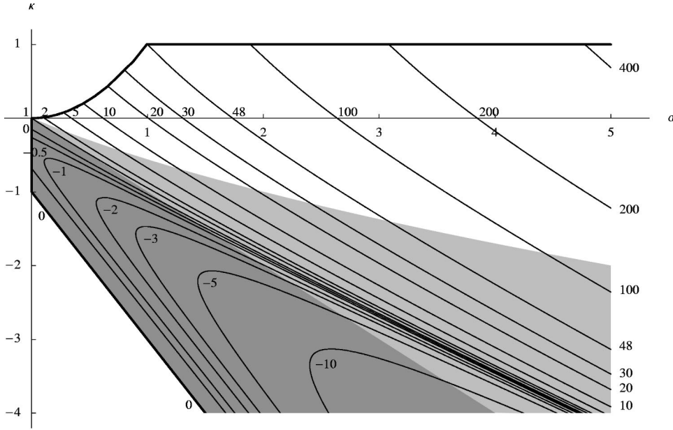
FIG. 4. Level lines for representative values of the magnetic moment m (measured in units of \frac{1}{3}\omega q R^2 ) in the physical region of the model parameters \alpha = M/2R and \kappa = (M^2 - q^2)/4R^2 . Concerning boundaries of the region, and gray shadows, see the caption of Fig. 1.
