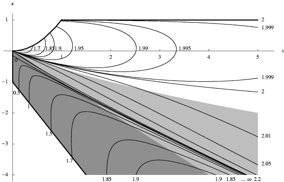
FIG. 5. Level lines for representative values of the gyromagnetic ratio G in the physical region of the model parameters \alpha = M/2R and \kappa = (M^2 - q^2)/4R^2 . Concerning boundaries of the region, and gray shadows, see the caption of Fig. 1.
